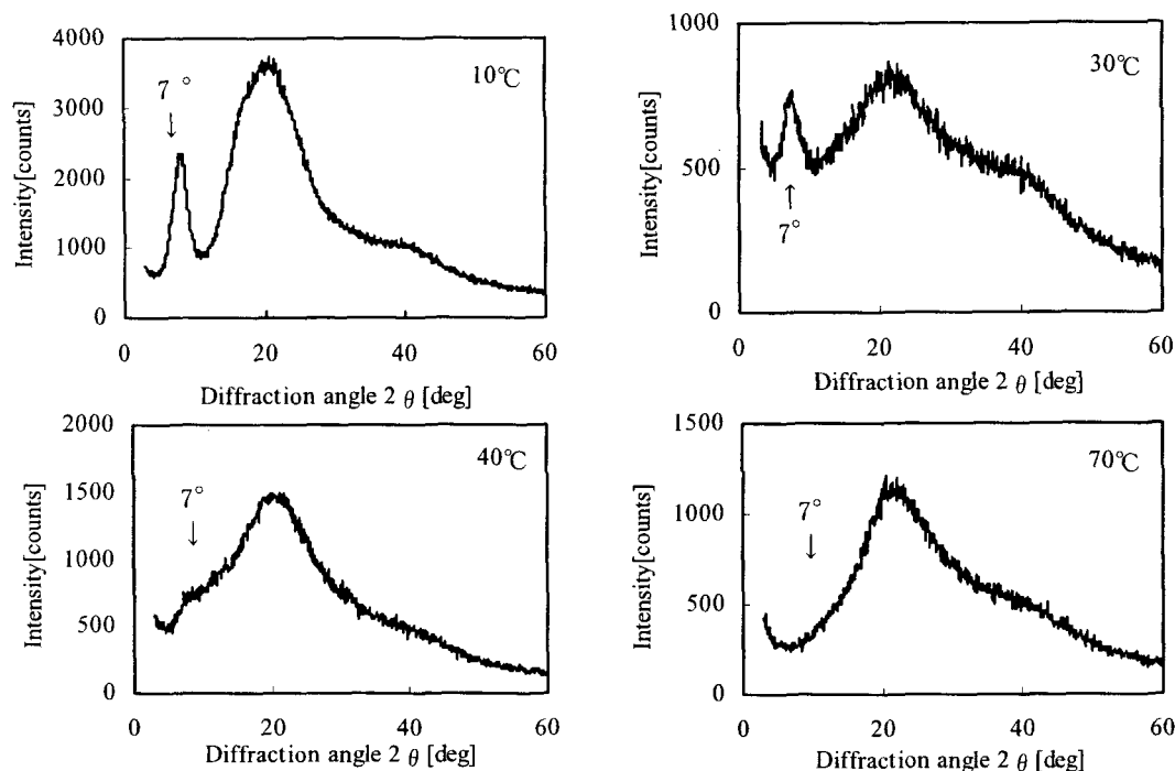
Fig.4 WAXD Patterns of The Dried Gelatin Prepared at Several Temperatures The sample was prepared by drying 10%(w/w) gelatin solution.
