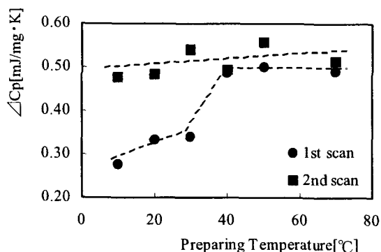
Fig.2 The Heat Capacity Increment \Delta C_p of The Dried Gelatin Prepared at Several Temperatures
