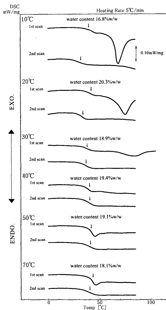
Fig.1 DSC Heating Curves for The Dried Gelatin Prepared at Several Temperatures The sample was prepared by drying 10%(w/w) gelatin solution.
